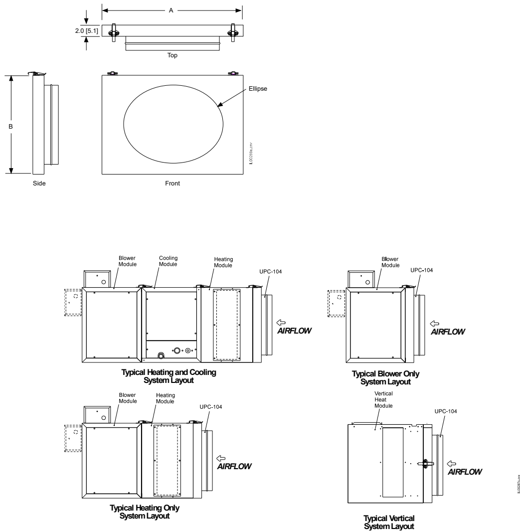
Figure 1. Typical Configurations with Heating Module Return Adapter
