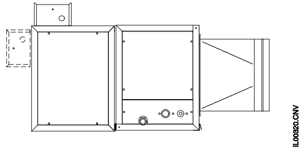
Figure 2. Typical Horizontal Modular System
