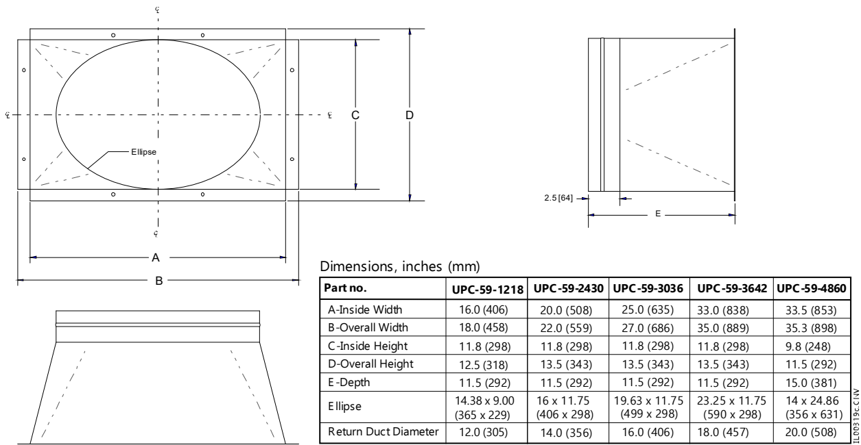
Figure 3. Dimensions of Cooling Module Return Air Adapter
